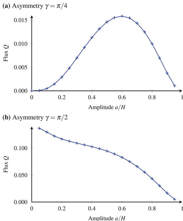
Fig. 4 The net flow rate through the channel, Q , as a function of its relative amplitude a/H in the case L/H = 2\pi . (a) Flux for \gamma = \pi/4 (as Fig. 3b), showing behaviour representative of weak asymmetry (unfolded) channels. (b) Flux for \gamma = \pi/2 (as Fig. 3d), showing distinct behaviour for strong asymmetry (folded) channels.
