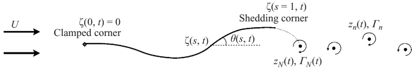
FIGURE 1. Vortex shedding behind a flapping flag. The oncoming flow is horizontal and vortices are shed from the trailing edge. The last vortex has unsteady intensity, the other vortices have frozen circulation.
