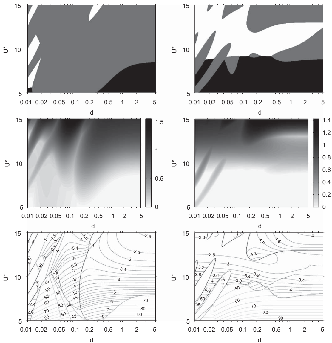
Fig. 6. Evolution of the dominant mode properties in the (d, U^*) -plane for M^* = 2 (left) and M^* = 4 (right). (Top) Regime observed (with the same color code as in Fig. 5). (Center) Growth rate of the most unstable mode (stable regions are indicated with a zero growth rate). (Bottom) Frequency of the dominant mode.
