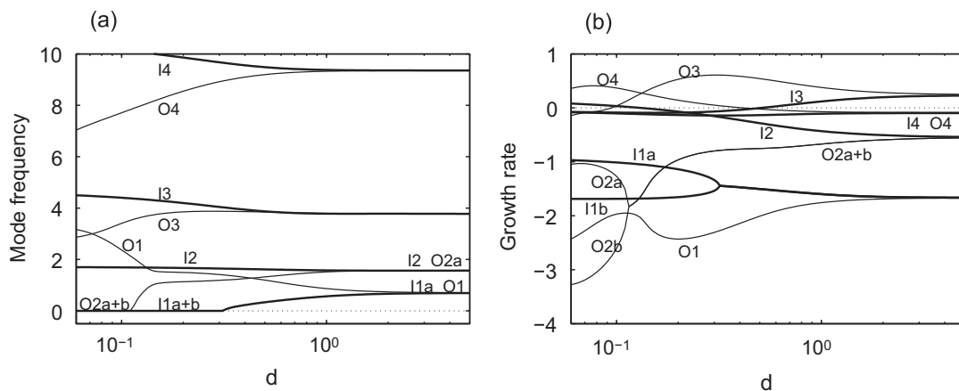
Fig. 9. Same as Fig. 8 for M^* = 2 and U^* = 10 .
