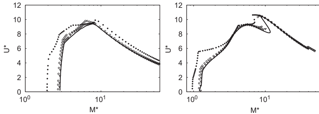
Fig. 13. Evolution of the critical stability curve in the (M^*, U^*) -plane for d = 0.2 (left) and d = 0.5 (right), and an increasing number of plates: N = 2 (stars), N = 5 (circles) and N = 10 (triangles). The limit N \rightarrow \infty described in Section 5.2 is plotted as a thick black line.
