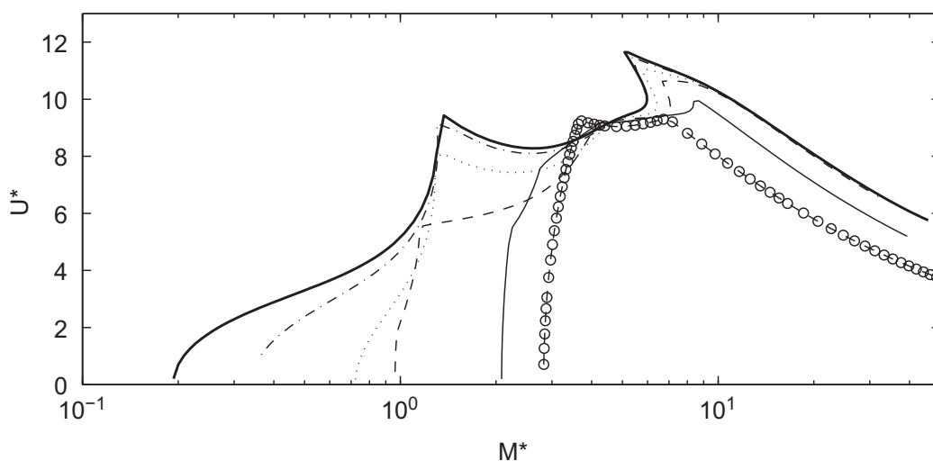
Fig. 4. Critical stability curve of the state of rest of two plates in the ( M^* , U^* )-plane for d = 0.1 (circle), d = 0.2 (thin solid), d = 0.5 (dashed), d = 1 (dotted) and d = 3 (dash-dotted). The thick solid line is the stability curve for one flag only using the same approach (Eloy et al., 2007) and is equivalent to d = \infty .
