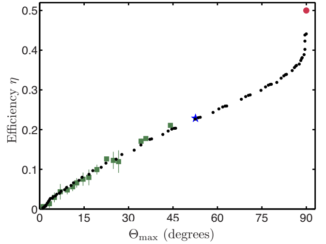
FIG. 14. (Color online) Final optimization diagram: optimal efficiency of the swimming stroke, \eta , as a function of the maximum Lagrangian angular displacement of the surface, \Theta_{\max} . Squares (green online): result from numerical optimization (the vertical and horizontal error bars denote the variability from the initial conditions and the weight of the constraint). Star (blue online): unconstrained optimal swimming stroke with \Theta_{\max} \approx 52.6^\circ and \eta \approx 22.2\% . Small black dots: envelope of the results obtained from the analytical ansatz for \sigma=0.1 and varying \beta and \gamma . Large circle (red online): asymptotic limit of the singular quasitreadmill swimmer of efficiency \eta=1/2 and maximum angular amplitude \Theta_{\max}=90^\circ .
