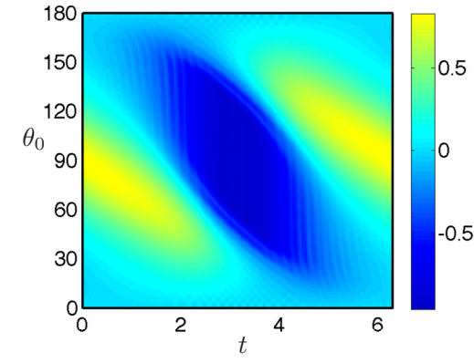
(a) Lagrangian velocity map
