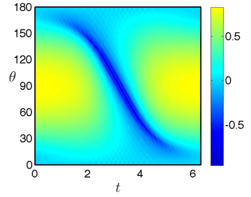
(a) Eulerian velocity map
