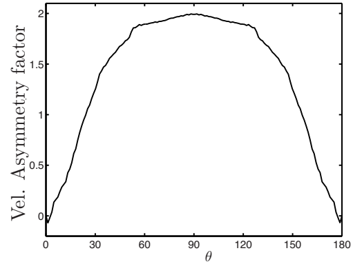
(b) Eulerian temporal asymmetry ratio
