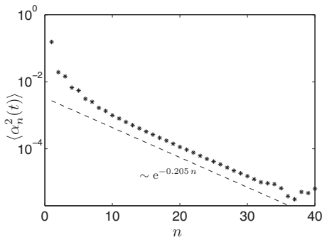
FIG. 3. The contribution of the successive modes, \langle \alpha_n^2 \rangle , to the efficiency (stars) decreases exponentially with the mode order, n . The results are plotted for the unconstrained optimization with efficiency \eta \approx 22.2\% and were obtained with M=40 , N_x=150 , and N_t=128 .
