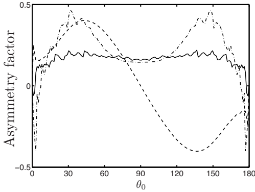
(b) Individual asymmetry
