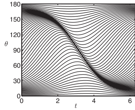
FIG. 4. Lagrangian description of the optimal swimming stroke with no constraint on the maximum displacement. The maximum amplitude of displacement is \Theta_{\max} \approx 52.6^\circ , the mean swimming velocity is \langle U \rangle \approx 0.33 , and the swimming efficiency is \eta \approx 22.2\% . Each curve illustrates the trajectory \theta = \vartheta(\theta_0, t) of a single material surface point.
