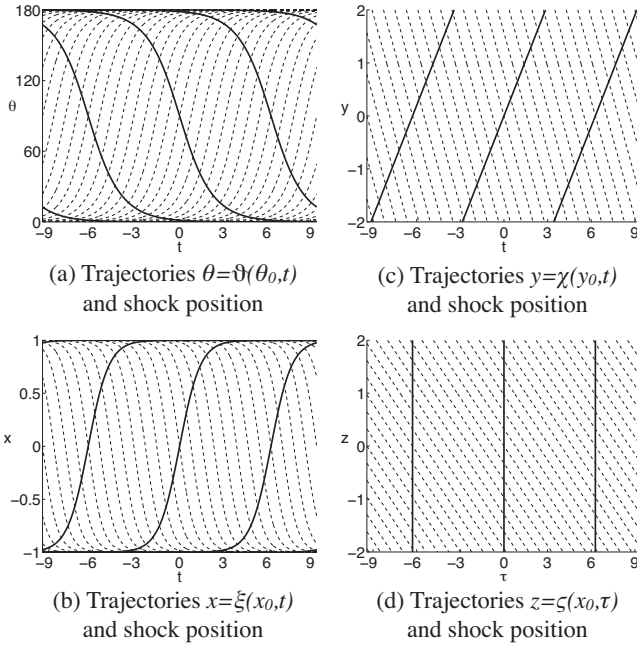
FIG. 12. The construction of the analytical ansatz is illustrated in the four successive coordinate systems used (a) (t, \theta) , (b) (t, x) , (c) (t, y) , and (d) (\tau, z) . The trajectories corresponding to the outer solution are shown in dashed lines and thick solid lines show the position of the shocks and inner solution trajectories [Eq. (55)]. Here, \gamma=1 and \beta=0.7 , and three swimming periods are shown.
