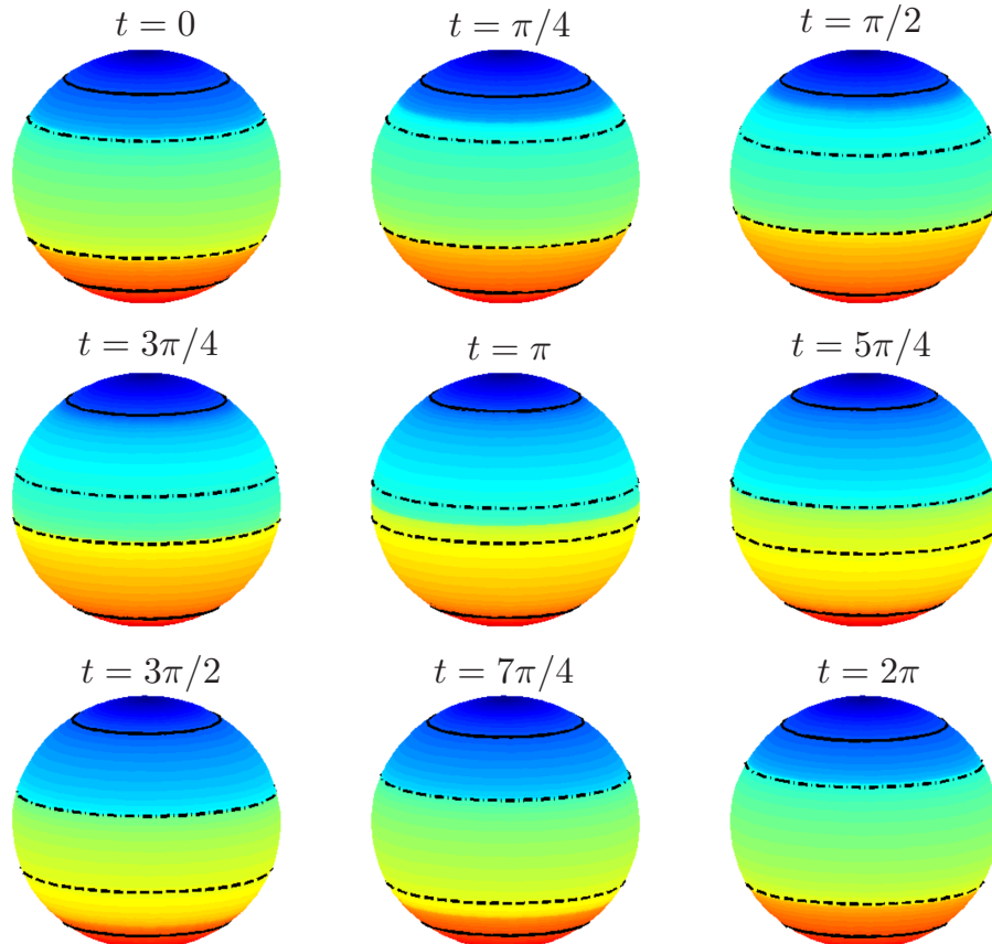
FIG. 9. (Color online) Same as Fig. 5 in the constrained case. The example illustrated here has a maximum displacement amplitude \Theta_{\max} \approx 10.6^\circ , a mean swimming velocity \langle U \rangle \approx 0.058 and a swimming efficiency \eta \approx 6.2\% .
