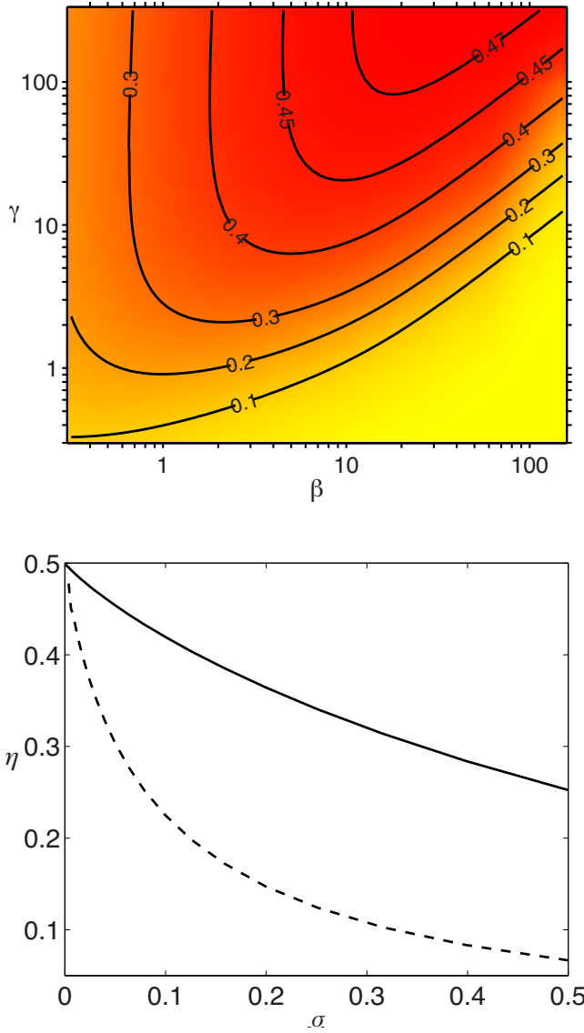
FIG. 13. (Color online) (Top) Variations of the swimming efficiency obtained for the analytical ansatz , for a sweep in the (\beta, \gamma) parameter space, and a shock width parameter of \sigma=0.05 ; lines display isovalues of \eta . (Bottom) Evolution with \sigma of the efficiency of the analytical ansatz for \gamma=1000 (solid) and \gamma=200 (dashed); in both cases \beta=800 .
