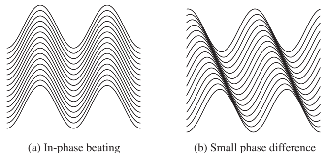
FIG. 7. A small phase difference between trajectories of neighboring Lagrangian points with identical and symmetric individual trajectories can lead to symmetry-breaking and the appearance of a shocklike structure. (a) Harmonic in-phase beating. (b) Same harmonic motion with a linearly spatially varying phase.
