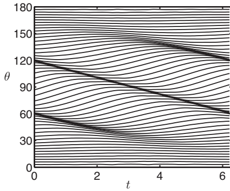
FIG. 8. Same as Fig. 4 in a constrained-displacement case. Here, the maximum displacement is \Theta_{\max} \approx 10.6^\circ , the mean swimming velocity is \langle U \rangle \approx 0.058 , and the swimming efficiency is \eta \approx 6.2\% .
