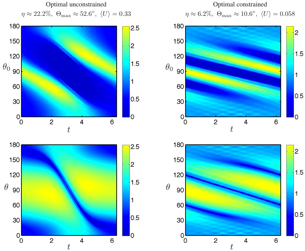
FIG. 15. (Color online) (Top) Lagrangian map in the (\theta_0, t) plane and (bottom) Eulerian map in the (\theta, t) plane of the stretching parameter S for the unconstrained swimming stroke (left) and the result of constrained optimization with efficiency 6.2% and maximum displacement 10.6^\circ (right).
