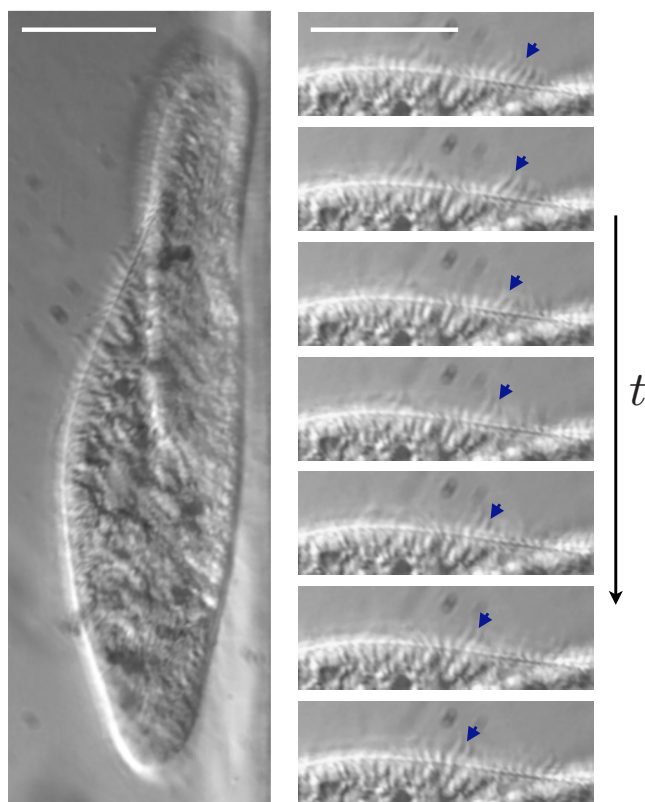
FIG. 1. (Color online) Paramecium swimming using metachronal waves (Hoffman modulation contrast microscopy, 40 \times magnification). Left: picture of the cell in a microchannel. Right: visualization of metachronal waves of cilia deformation propagating along the cell. Time increases from top to bottom, with a time difference of 1/300 s between each picture. Arrows indicate the propagation of a wave of effective strokes in the cilia array. The scale bar is 50 \mu m in both pictures. Pictures courtesy of Sunghwan (Sunny) Jung, Virginia Tech.
