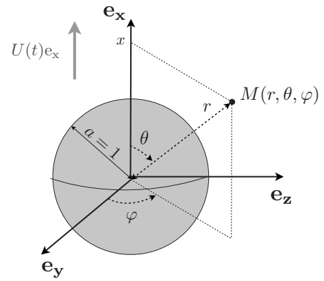
FIG. 2. Notation for the squirmer model. A comoving frame centered on the squirmer center is used with spherical polar coordinates (r, \theta, \varphi) . The axisymmetry of the surface motion imposes a purely translating swimming motion along \mathbf{e}_x with time-varying velocity U(t) . See text for details.
