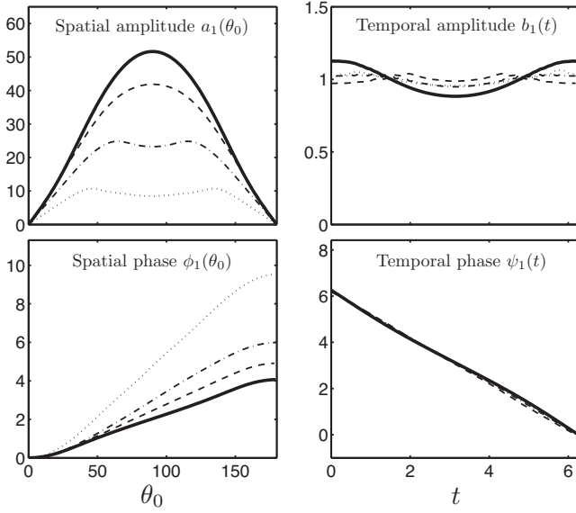
FIG. 18. Amplitude and phase characteristics of the dominant CEOF mode in the unconstrained swimming stroke of maximum efficiency (thick solid line: \Theta_{\max} \approx 52.6^\circ and \eta \approx 22.2\% ) and in constrained optimal strokes (thin lines): \Theta_{\max} \approx 44^\circ and \eta \approx 21\% (dashed), \Theta_{\max} \approx 25^\circ and \eta \approx 12.5\% (dashed-dotted), \Theta_{\max} \approx 11^\circ and \eta \approx 6.8\% (dotted).
