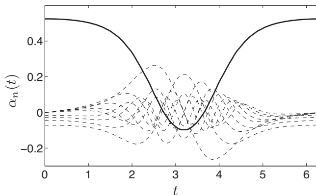
FIG. 6. Time-evolution of the ten first modes, \alpha_n(t) ( n \leq 10 ), over the period for the optimal unconstrained stroke shown in Fig. 5. The swimming mode or swimming velocity U(t) = \alpha_1(t) is plotted as a thick solid line. Modes 2 through 10 are plotted as dashed line. The swimming mode is observed to dominate during the effective stroke (for t \leq \pi/2 and t \geq 3\pi/2 ), while many modes are significant during the recovery stroke ( \pi/2 \leq t \leq 3\pi/2 ).
