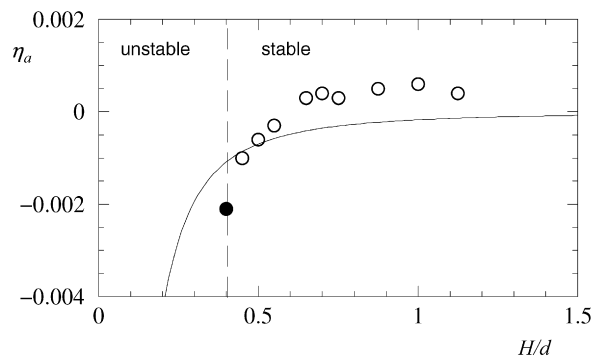
Fig. 3. Comparison of measurements (O stable, ● unstable) and predictions (—), Eq. (6a) of the added damping for the circular jet.
