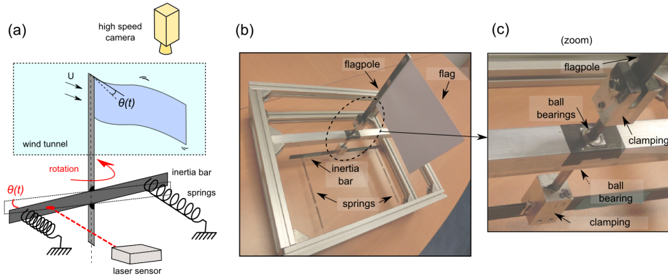
Figure 1: Experimental set-up. (a) Schematic representation of the experiment. The flagpole is attached to a spring-mass oscillator, which is out of wind-tunnel. A laser sensor measures the angle of rotation \theta of the rotating inertia bar fixed to the flagpole. (b,c) Photographs of the experimental set-up (here the whole system is out of wind-tunnel), where it can be seen that the flagpole is guided by ball bearings.
