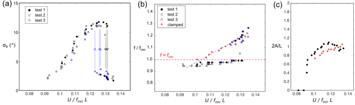
Figure 4: Analysis of reproducibility (case of a steel flag). Values obtained by gradually increasing the wind velocity are superimposed with values obtained by gradually decreasing the wind velocity (blue color) and "test 1", "test 2", "test 3" denote the independent reproducibility tests made under the same experimental conditions. (a) Evolution of the standard deviation \sigma_\theta of the angle of rotation of the flagpole as a function of the reduced wind velocity. (b) Dominant frequency of the flagpole oscillation. The natural frequency of the oscillator is indicated by the dotted horizontal line ( f_{osc} = 8.2 Hz). The expected trend of the flapping frequency without lock-in is suggested by the gray dotted line, supported by experimental data measured at decreasing wind velocity (crosses). (c) Evolution of the amplitude peak-to-peak of the trailing edge of the flag in the coupled configuration (circles) and clamped (crosses), normalized by the flag length L .
