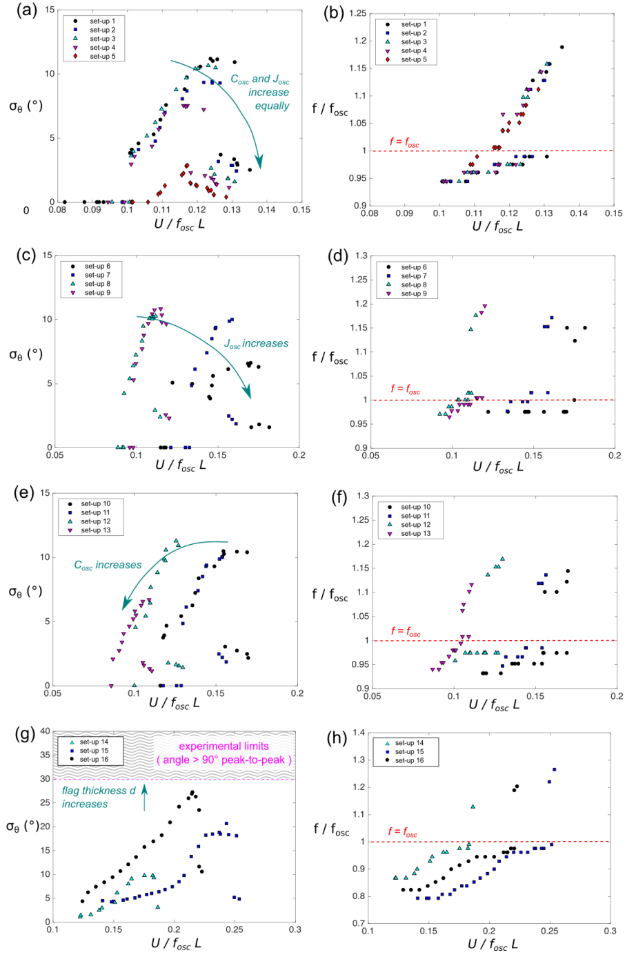
Figure 5: Amplitude and frequency of the rotation of the flagpole for several parameters of coupling. The natural frequency of the oscillator is adjusted to be very slightly above the flapping frequency of the flag at the threshold of flutter instability. Values obtained by gradually increasing the wind velocity are superimposed with values obtained by gradually decreasing the wind velocity. (a,b) With variations of C_{osc} and J_{osc} (in the same proportions). (c,d) With variations of J_{osc} and L . (e,f) With variations of C_{osc} and L . (g,h) With variations of d and L .
