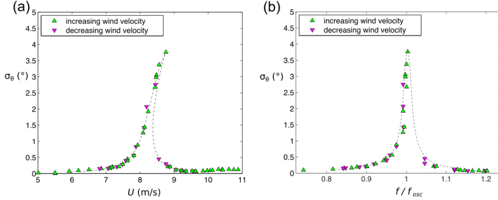
Figure 3: Evolution of the fluctuations of \theta(t) , characterized by the standard deviation \sigma_\theta (case of a paper flag). For each datapoint at a precise wind velocity, we wait about three minutes before recording, in order to not be affected by any transient signal. (a) We can think of a bent-over resonance curve when it is plotted as a function of the wind velocity. (b) Nevertheless, we observe a classical resonance curve as a function of the flapping frequency of the flag. The dotted lines are guides for the eyes.
